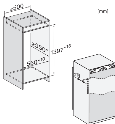
K7433E, K7434E, K7464E, K7443D, K7444D, K7473D, K7474D, FNS7470D, Einbau (Fußnote*) (Skizze)
