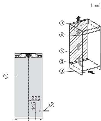
K7433E, K7434E, K7464E, K7443D, K7444D, K7473D, K7474D, FNS7470D, Installation (Fußnote*) (Skizze)
