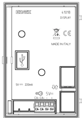
Backside view
