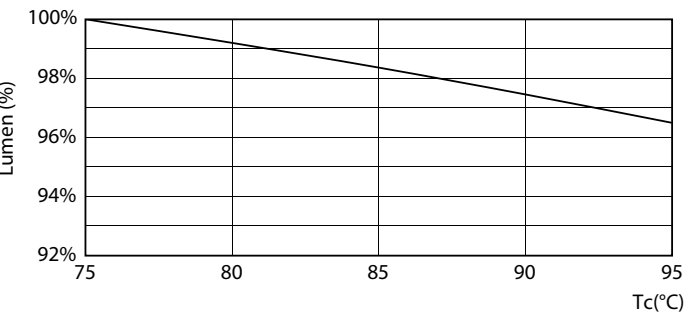
LEDtube MAS EU 36W 60K LumenVsTc-LMP
