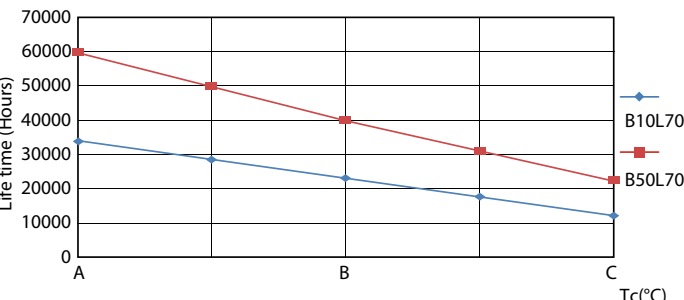
LEDtube_60K_LifetimeVsTc
