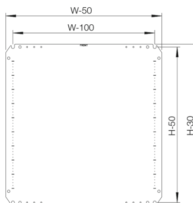
Mounting plate
