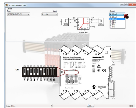
example for DIP switch setting with software tool
