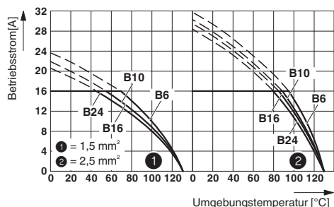
Derating-Diagramm
